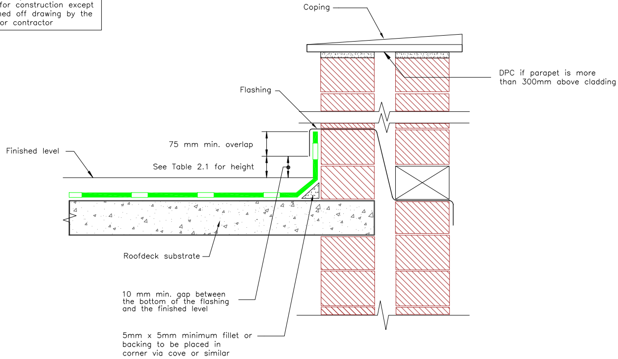
Cavity wall detail
